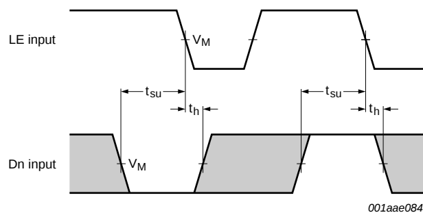
Fig 11. Set-up and hold time data input (Dn) to latch enable input (LE)
